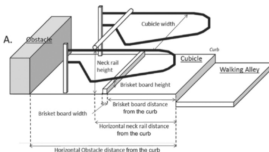
Figure 3: Schematic representation of important cubicle design criteria (© 2023 Elsevier inc.)
