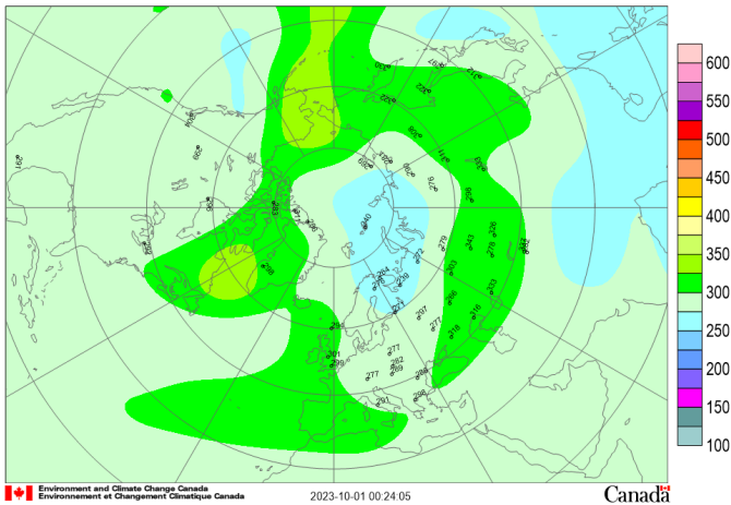
Mean total ozone (DU), 2023/09/01-2023/09/30
